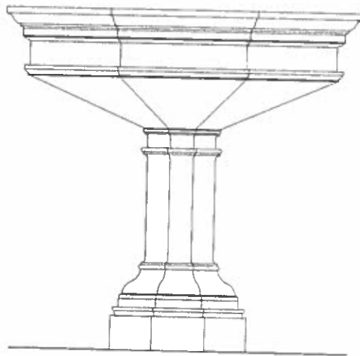
1 BAPTISMAL FONT ELEVATION 14.12 1 1/2" = 1'-0"
